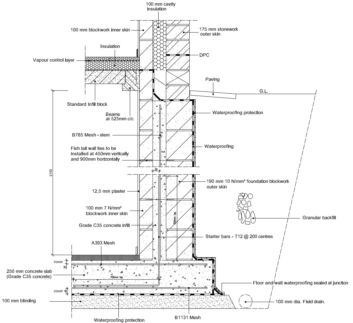
BASEMENT DETAIL (1:10)
